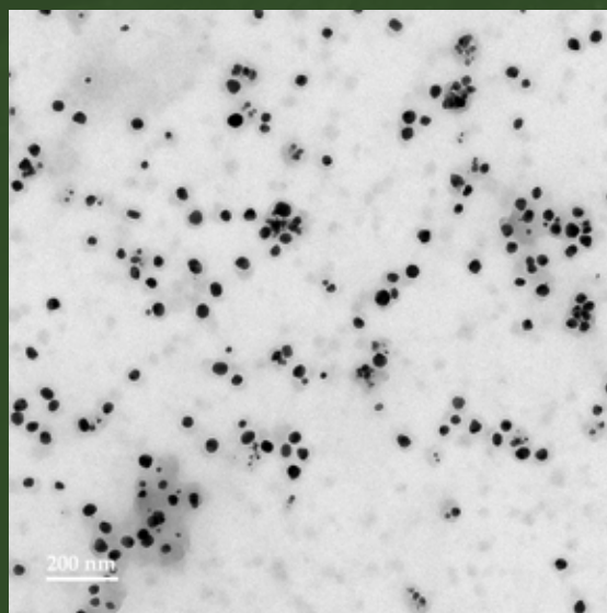
TEM Image of KDM-AG-00001
