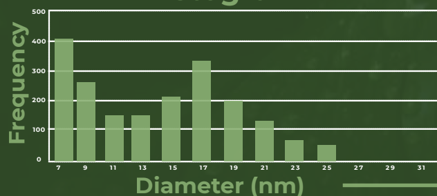
Histogram
