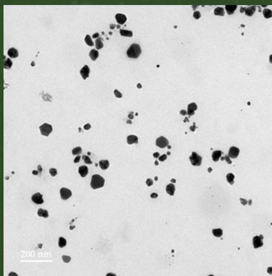
TEM Image of BRJ-AG-00194
