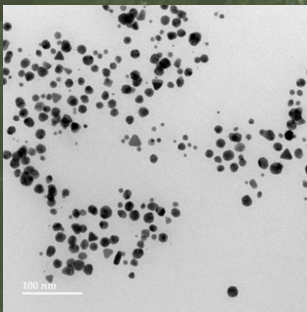
TEM Image of MND-AU-00019
