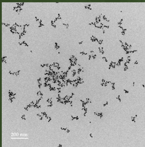
TEM Image of VDK-AU-00062
