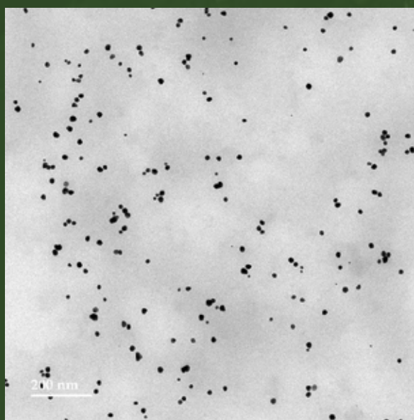
TEM Image of CIC-AU-00076
