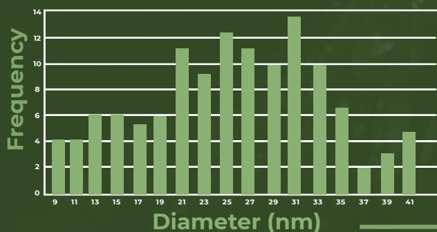
Histogram
