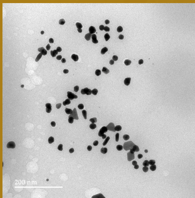
TEM Image of BFR-AU-00193
